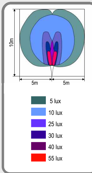
Isolux diagram
